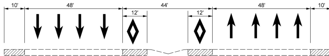
Figure A-5 Shoulder Use (portion) Section
