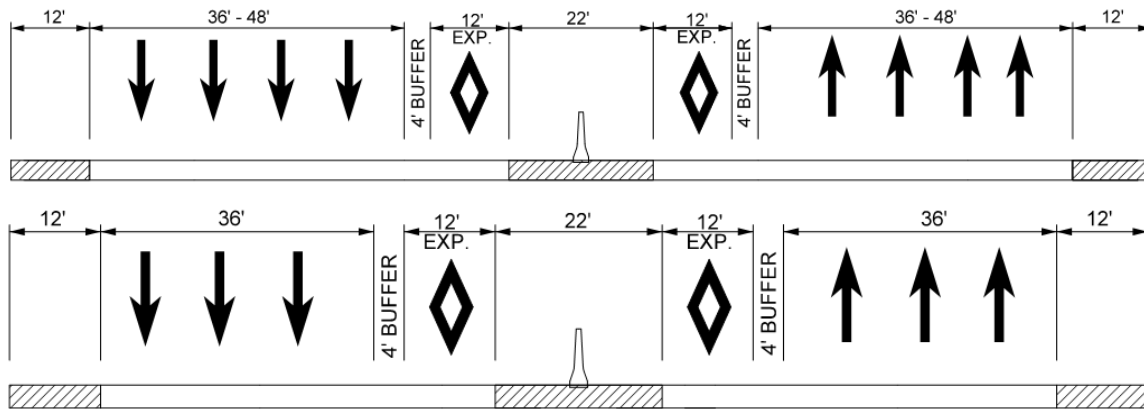
Figure A-20 Full Feature Section
