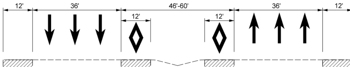
Figure A-15 Shoulder Use Option Section
