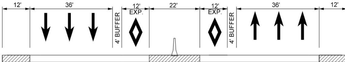
Figure A-32 Full Feature Section
