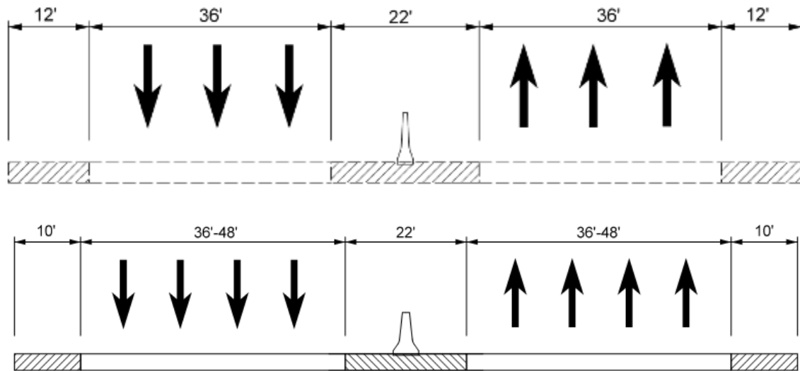
Figure A-18 Existing Typical Section
