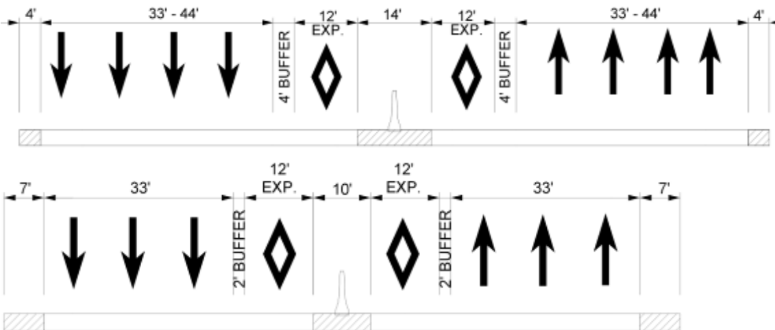
Figure A-19 Constrained Section
