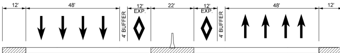
Figure A-26 Full Feature Section
