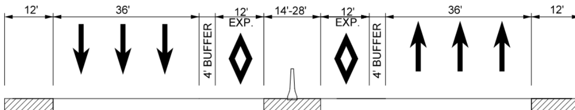
Figure A-16 Constrained Section
