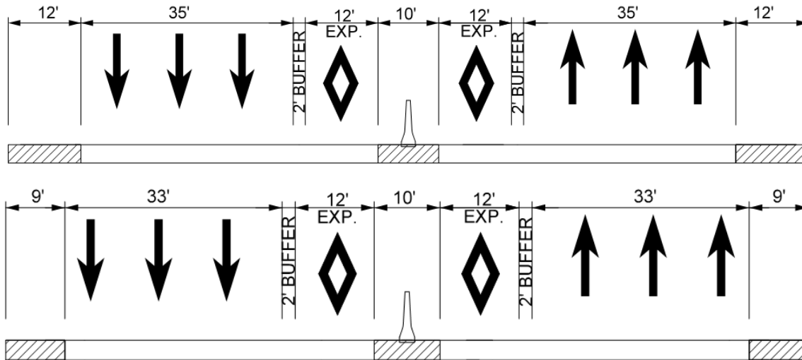
Figure A-28 Constrained Section
