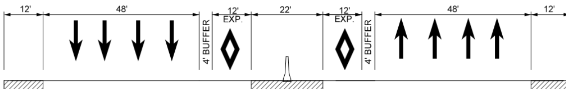
Figure A-23 Full Feature Section
