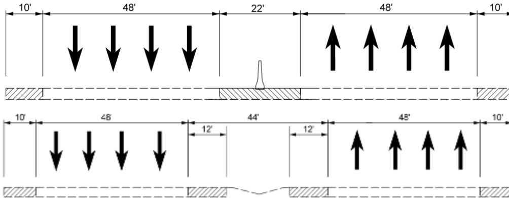
Figure A-4 Existing Typical Section
