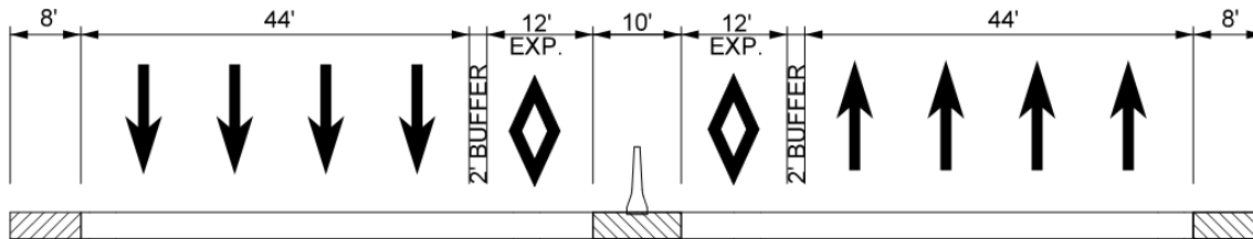
Figure A-9 Constrained Cross Section
