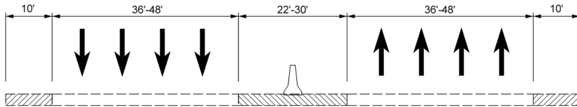
Figure A-11 Existing Typical Section
