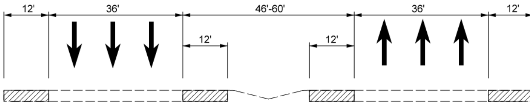
Figure A-14 Existing Typical Section
