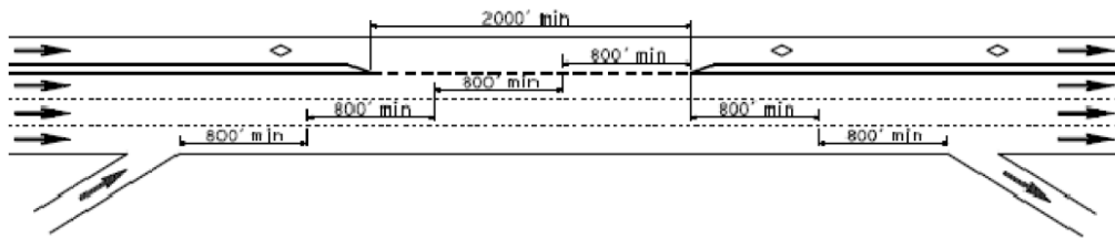
Figure 4-6: Weave-Zone Access Design
