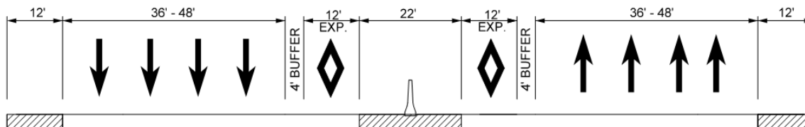
Figure A-13 Full Feature Section
