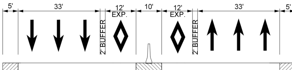
Figure A-2 Constrained Section
