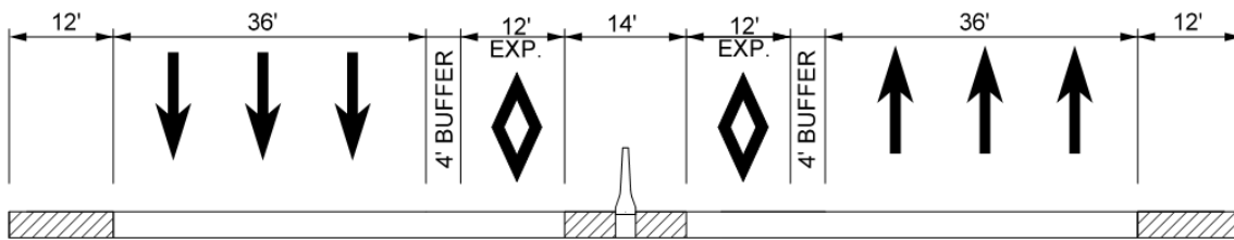
Figure A-31 Constrained Section
