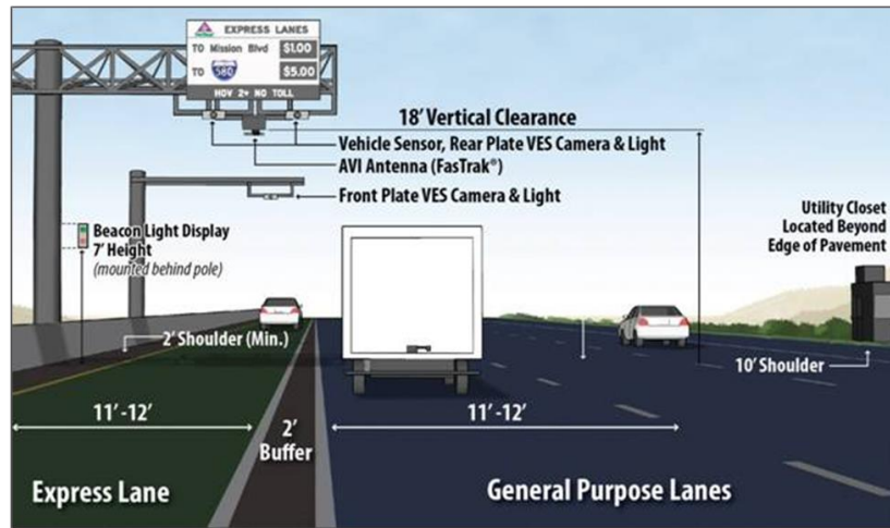
Figure 4-10: Typical Toll Zone Design
