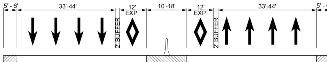
Figure A-12 Constrained Section
