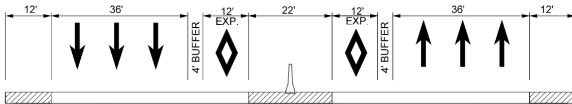
Figure A-29 Full Feature Section
