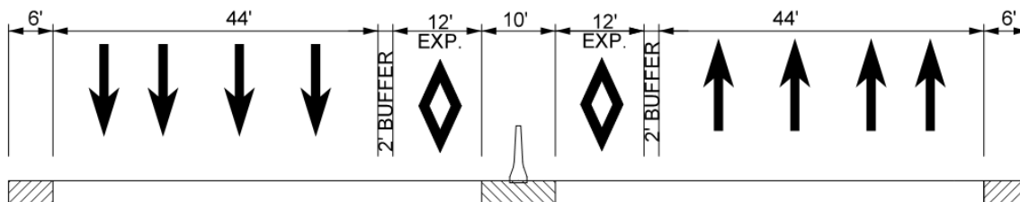
Figure A-22 Constrained Section
