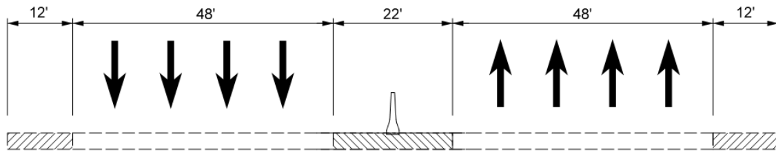
Figure A-8 Existing Typical Section
