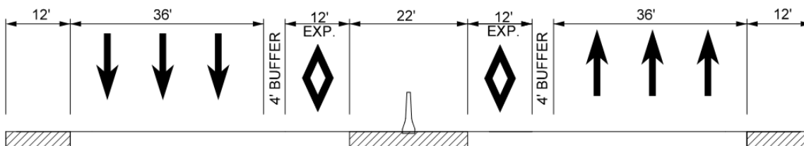
Figure A-17 Full Feature Section
