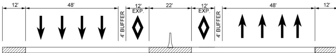
Figure A-7 Full Feature Section
