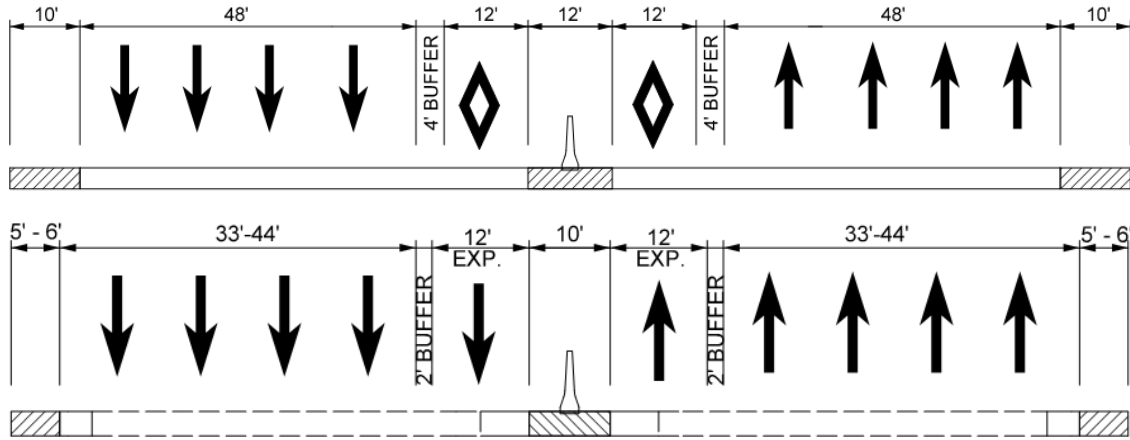
Figure A-6 Constrained Section
