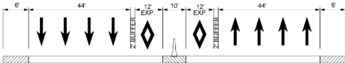
Figure A-25 Constrained Section
